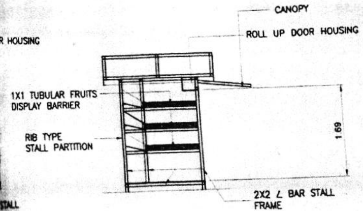
SECTION THRU - B SCALE 1:60M.
