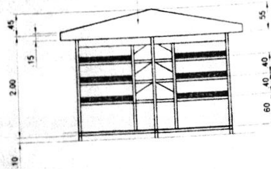
SIDE ELEVATION SCALE 1:60M.
