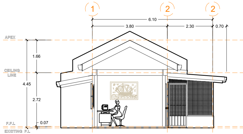
SECTION THRU Y SCALE 1:100m
