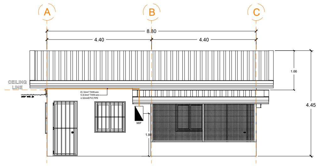
SERVICE ENTRANCE SCALE
