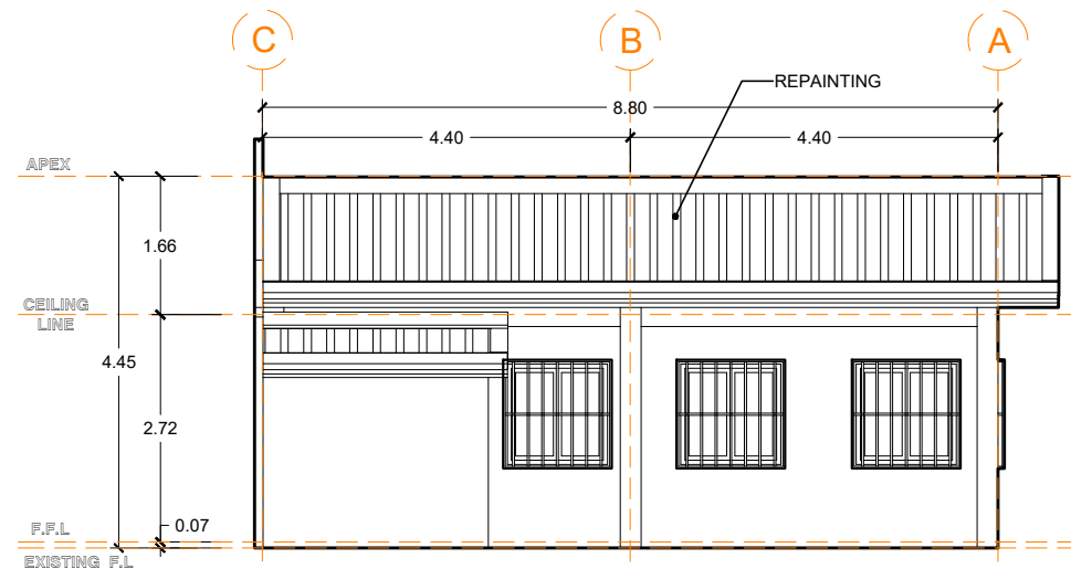
REAR ELEVATION SCALE 1:100m
