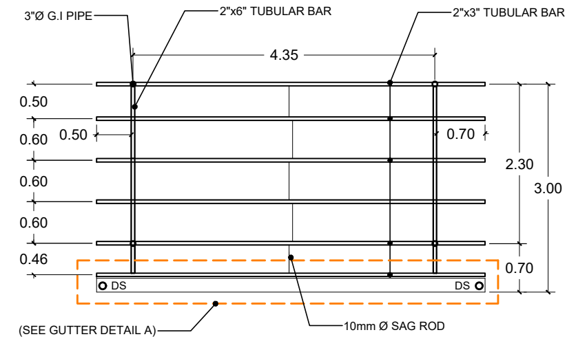
ROOF FRAMING PLAN SCALE 1:75m
