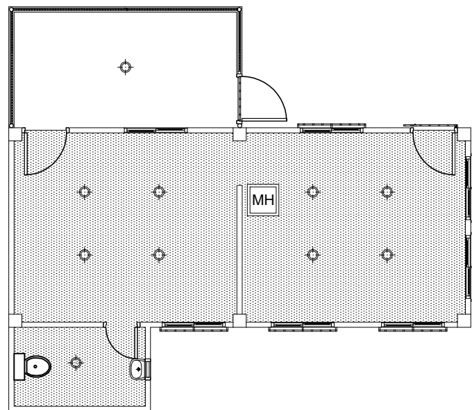
REFLECTED CEILING PLAN SCALE 1:100m
