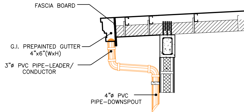
ROOF GUTTER DETAIL B
