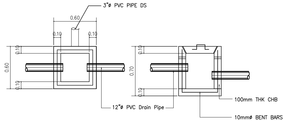
CATCH BASIN PLAN & SECTION
