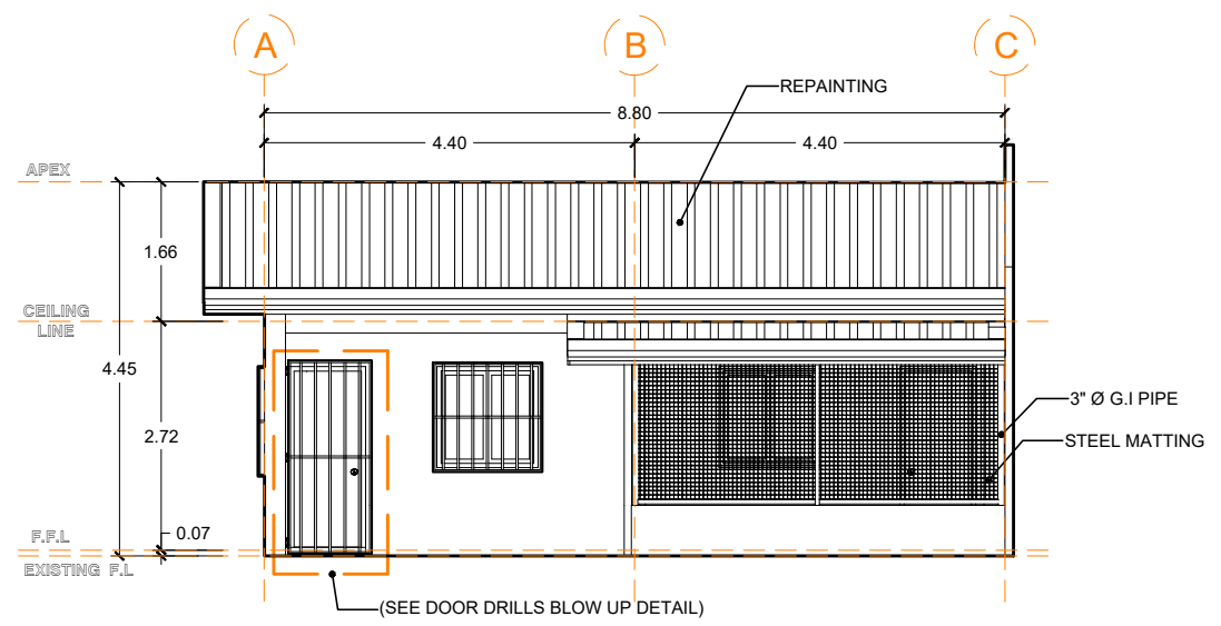
FRONT ELEVATION SCALE 1:100m
