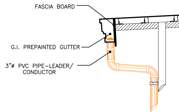
ROOF GUTTER DETAIL A
