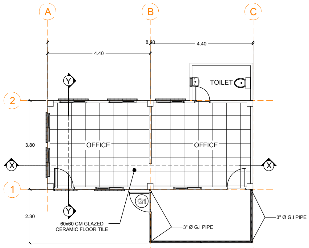
FLOOR PLAN SCALE 1:100m
