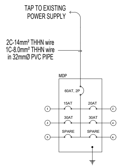
RISER DIAGRAM NTS
