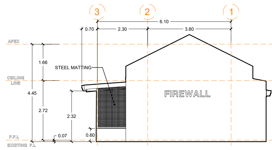
RIGHT-SIDE ELEVATION SCALE 1:100m
