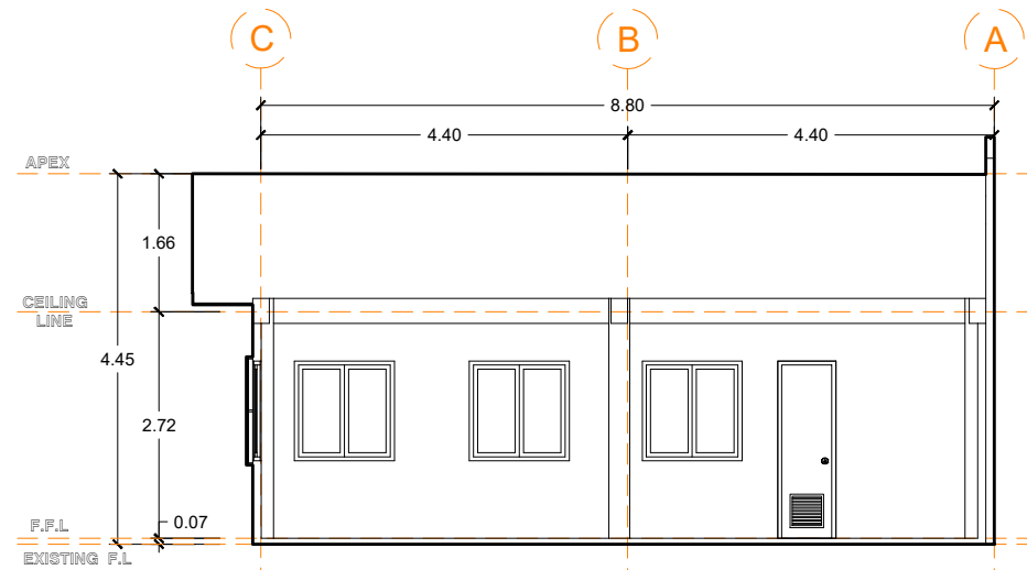
SECTION THRU X SCALE 1:100m
