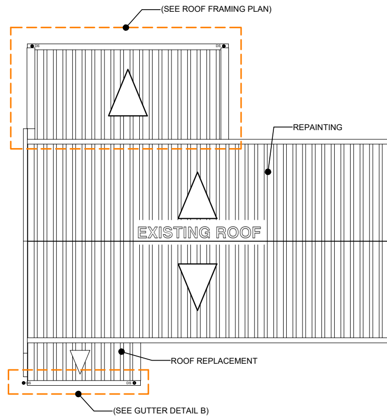
ROOF PLAN SCALE 1:100m
