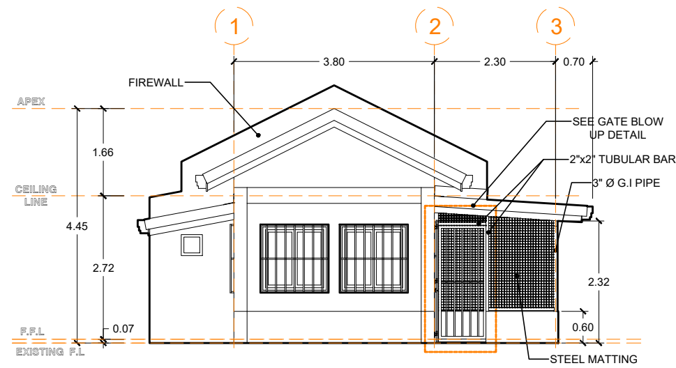
LEFT-SIDE ELEVATION SCALE 1:100m
