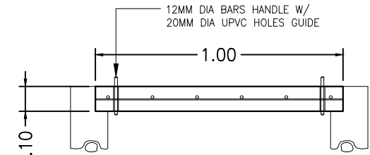
MANHOLE COVER PLAN SCALE 1:30m
