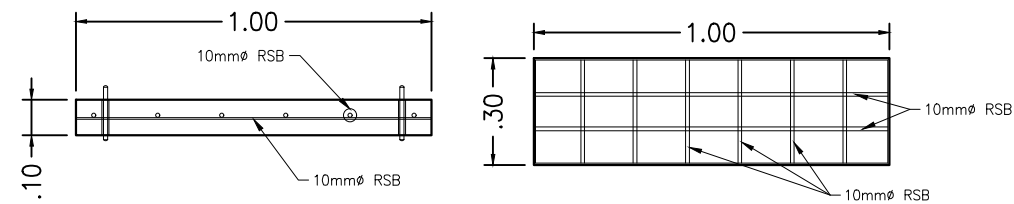
MANHOLE COVER REBARS SCALE 1:20m
