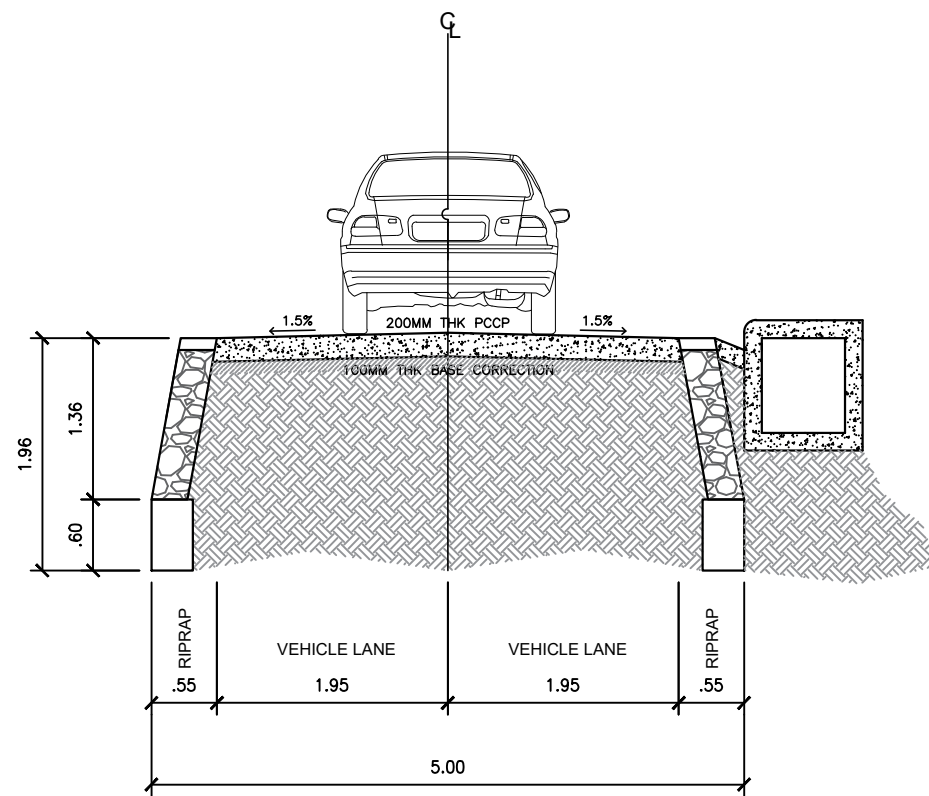
ROAD (LOT-3) SECTION SCALE 1:60m
