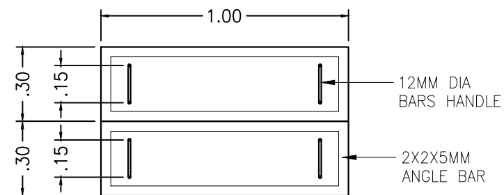
MANHOLE COVER PLAN SCALE 1:30m
