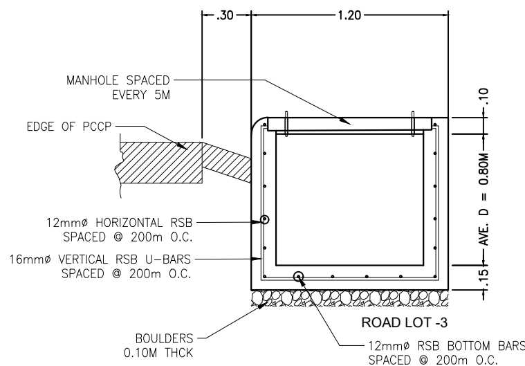
DRAINAGE W/ SIDEWALK SECTION SCALE 1:30m
