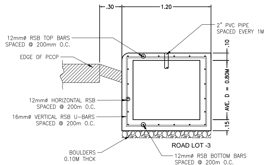
DRAINAGE W/ SIDEWALK SECTION SCALE 1:30m
