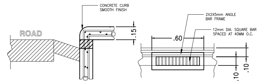
DRAIN INLET DETAIL SCALE 1:30m
