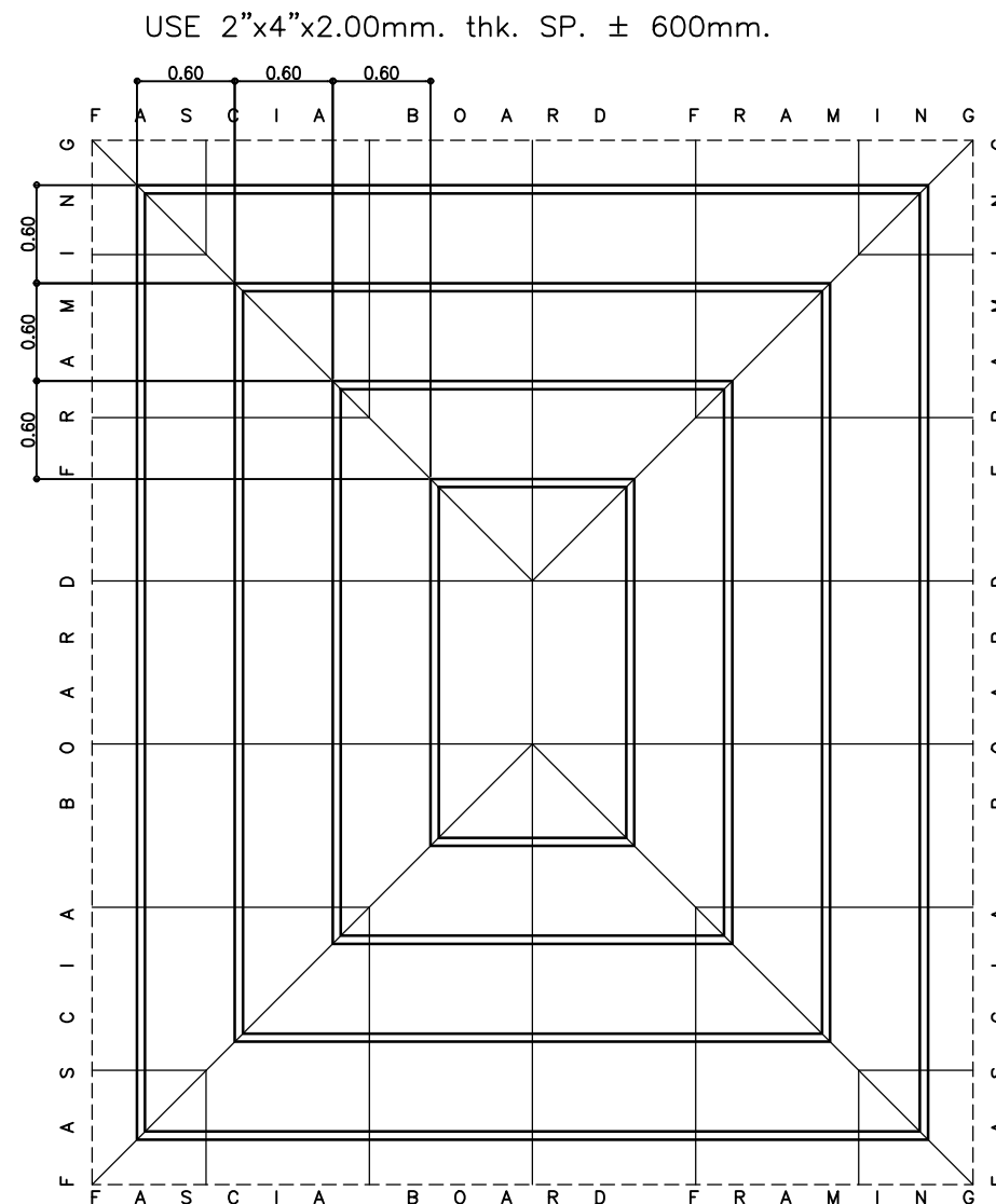
PURLIN LAYOUT PLAN SCALE 1:100M.
