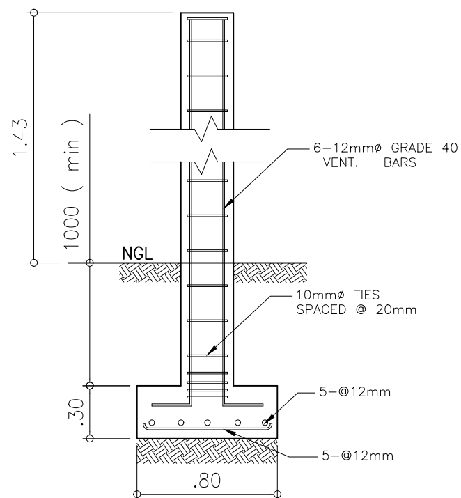
C1-F1 DETAIL SCALE 1:30M
