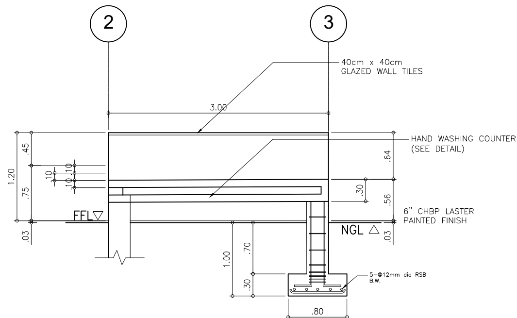
LONGITUDINAL SECTION DETAILS SCALE 1:50M
