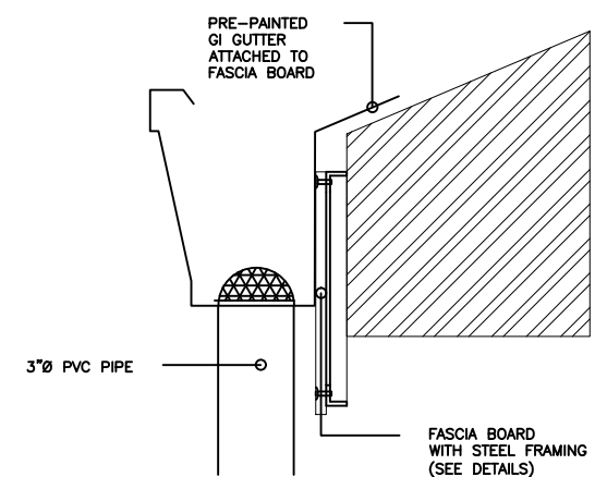
GUTTER DETAIL SCALE 1:10M.
