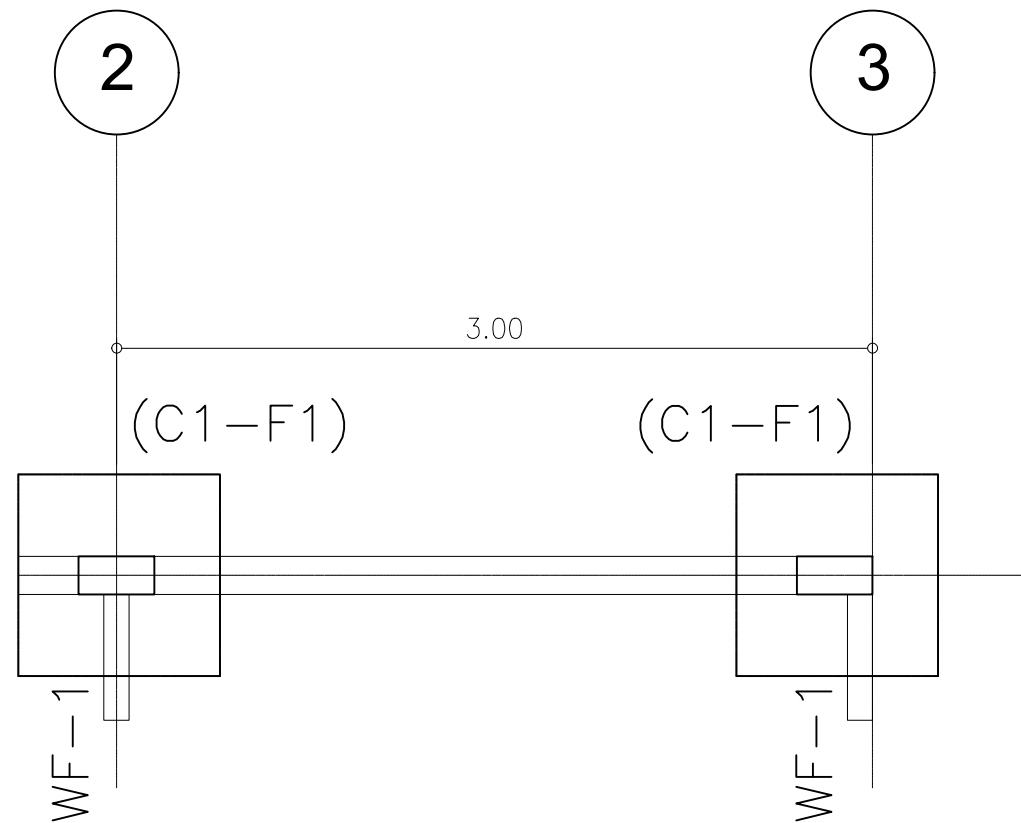
FOUNDATION PLAN SCALE 1:30M
