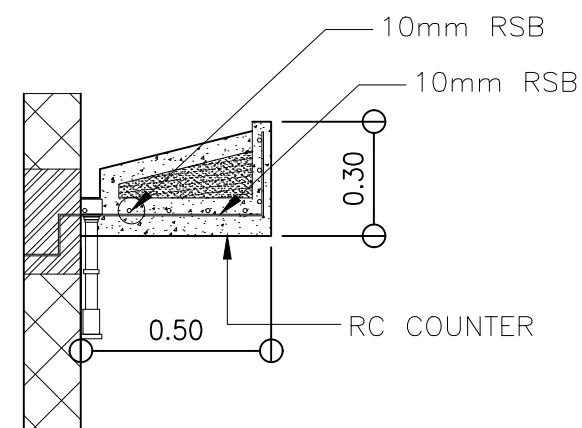
HANDWASHING COUNTER DETAILS SCALE 1:100M
