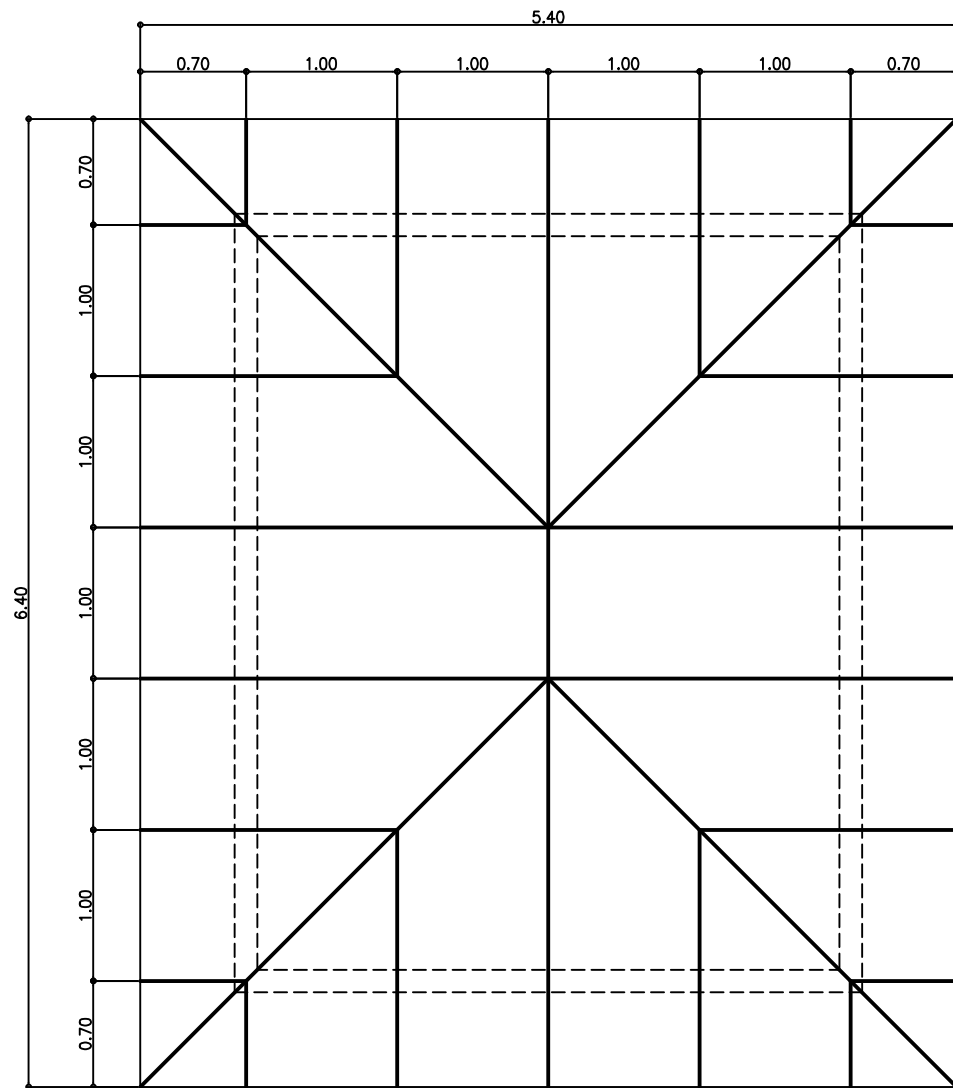
ROOF FRAMING PLAN SCALE 1:100M.
