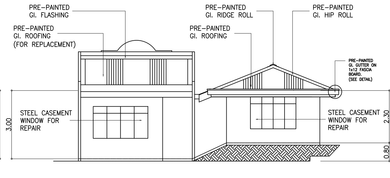
REAR ELEVATION SCALE 1:100M.
