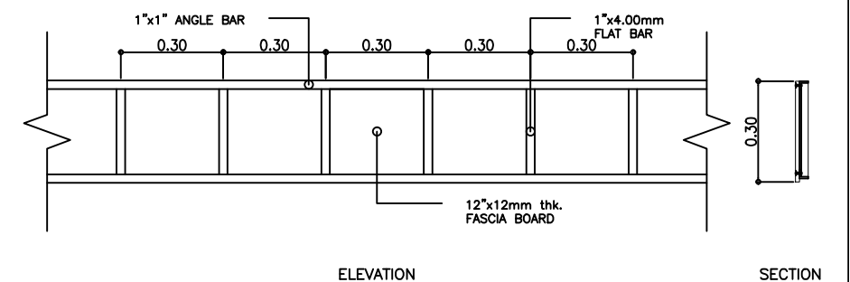
FASCIA BOARD FRAMING DETAIL SCALE 1:20M.
