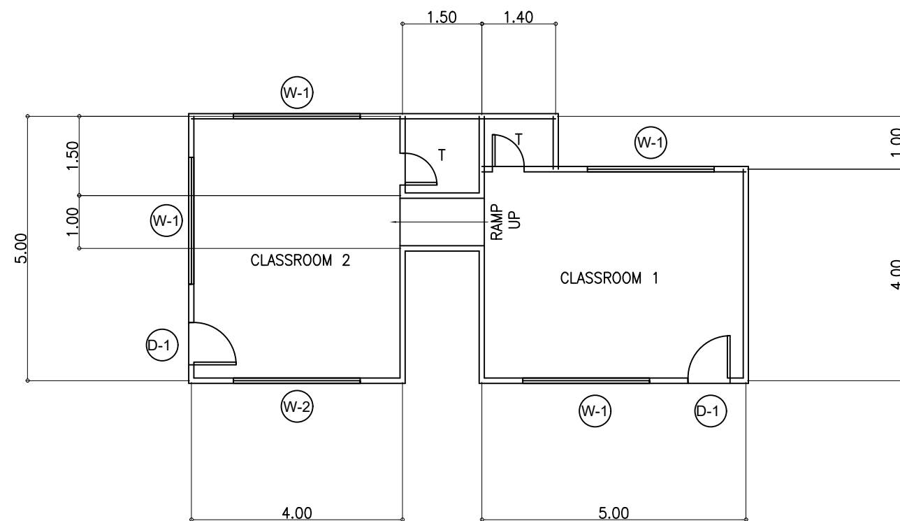
FLOOR PLAN SCALE 1:100M.
