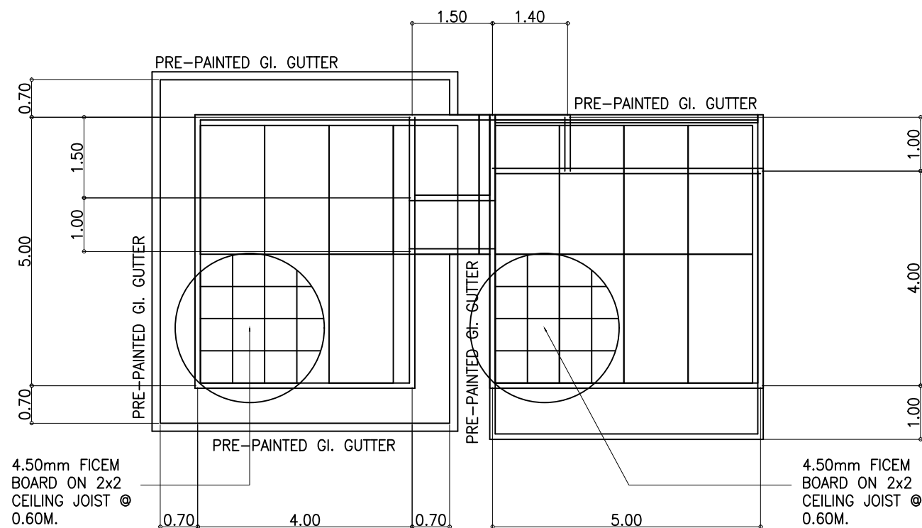
REFLECTED CEILING PLAN SCALE 1:100M.
