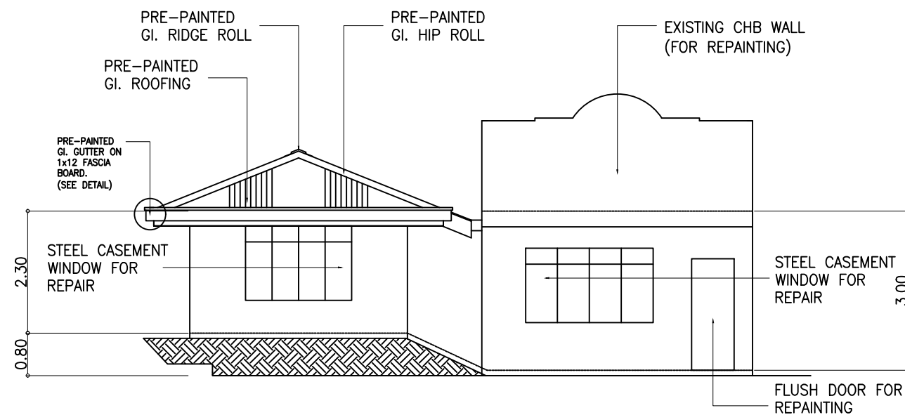
FRONT ELEVATION SCALE 1:100M.
