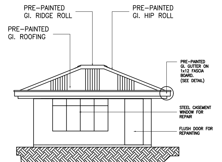
LEFT SIDE ELEVATION SCALE 1:100M.
