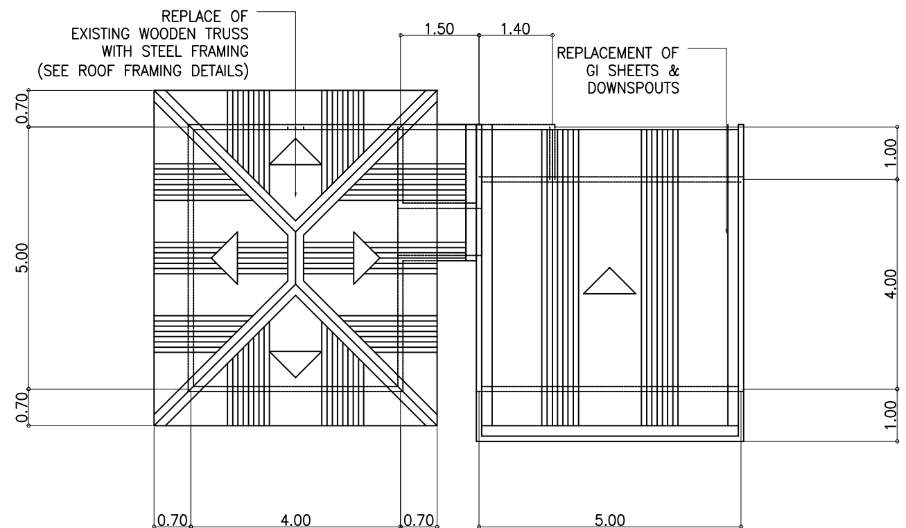
ROOF PLAN SCALE 1:100M.
