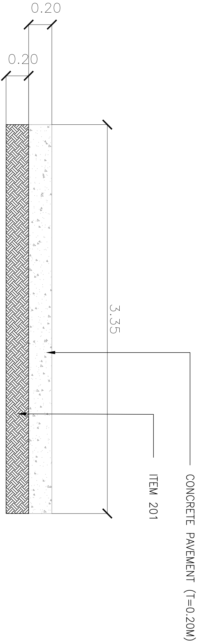
PAVEMENT SECTION
