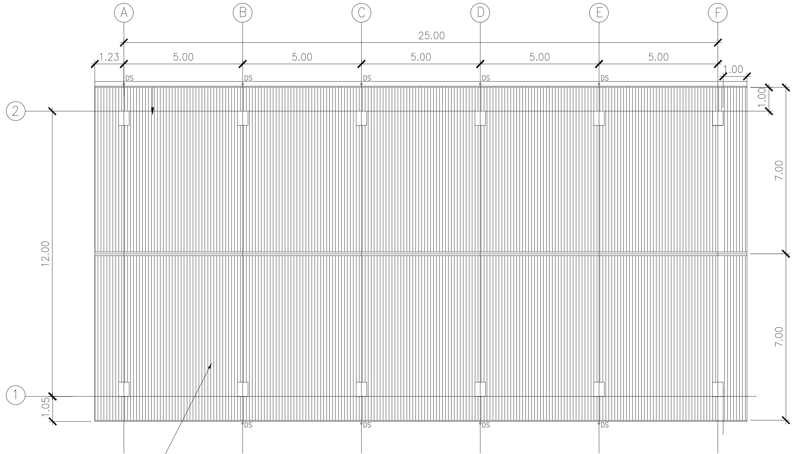
SITE DEVELOPMENT PLAN SCALE 1:150
